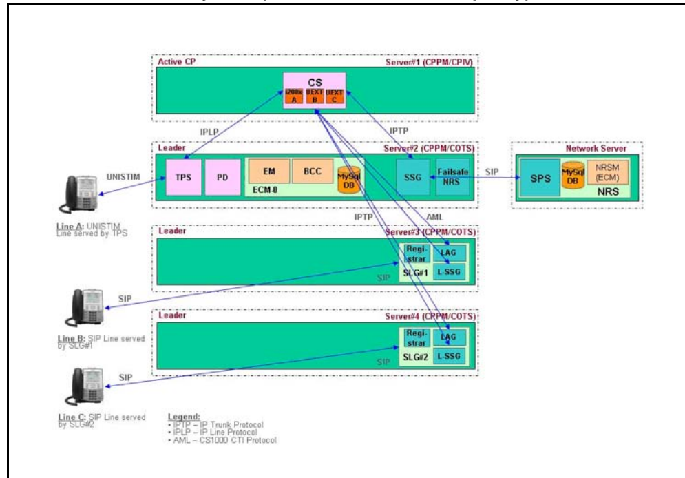
Figure 5 Four-server CS 1000 system (with double SIP Line capacity)
