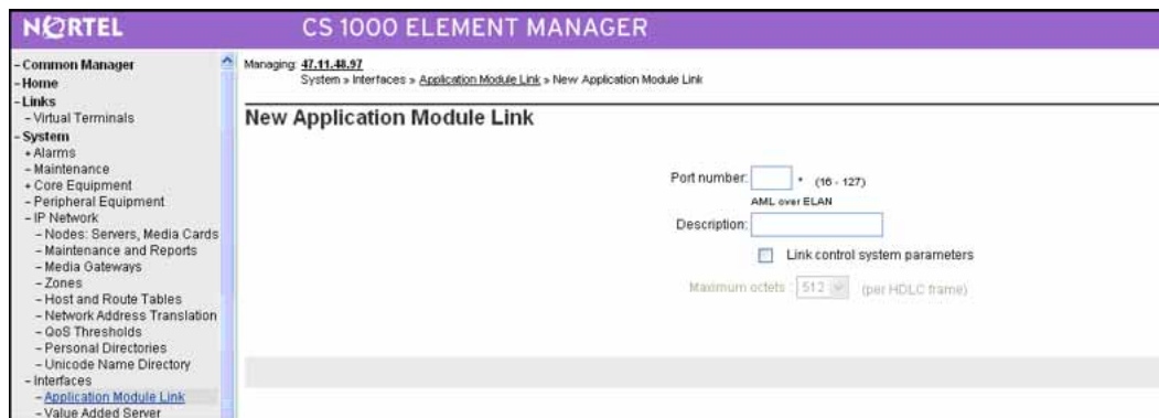
Figure 19 New Application Module Link
