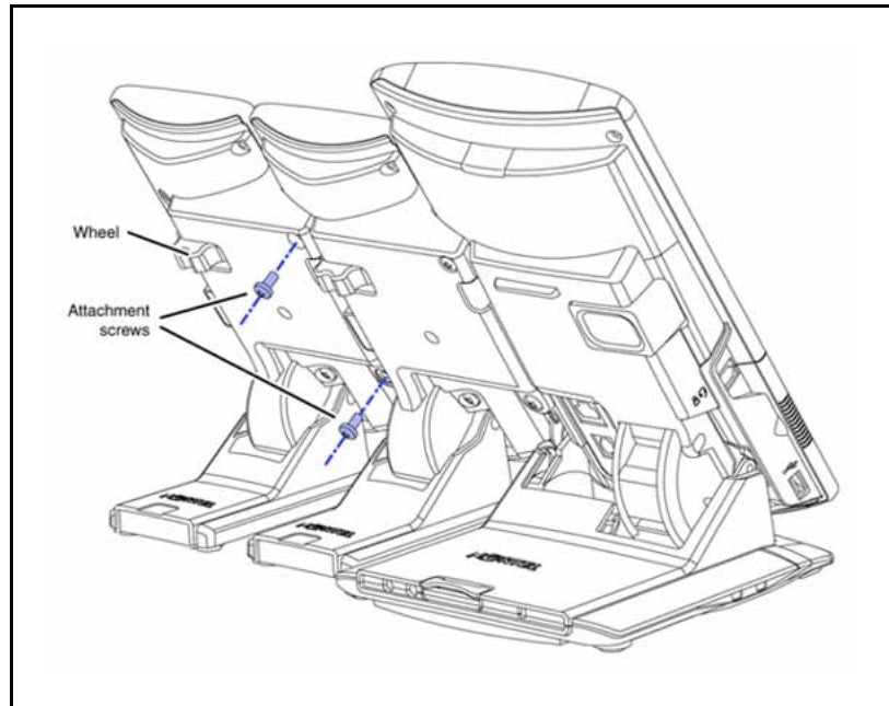
Figure 68 Connecting the Expansion Module
