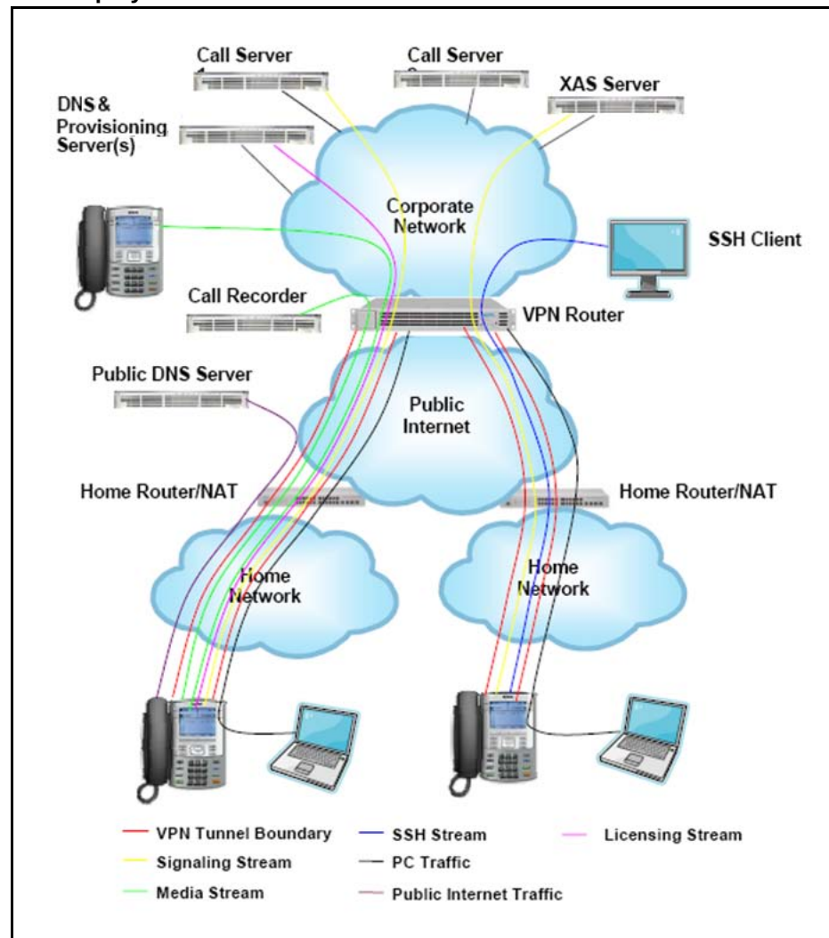
Figure 83 VPN deployment model
