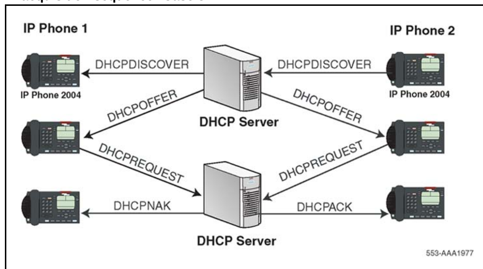
Figure 73 IP acquisition sequence: Case 3
