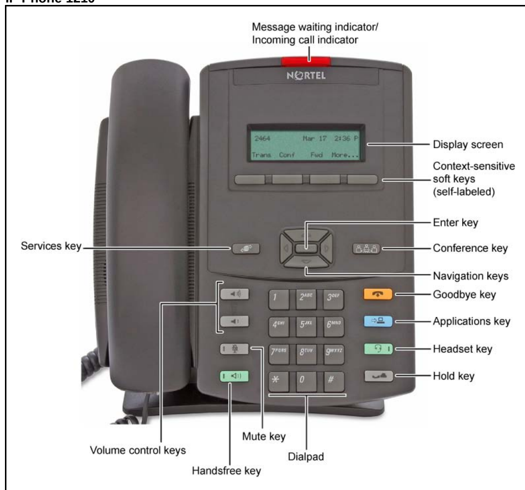
Figure 22 IP Phone 1210
