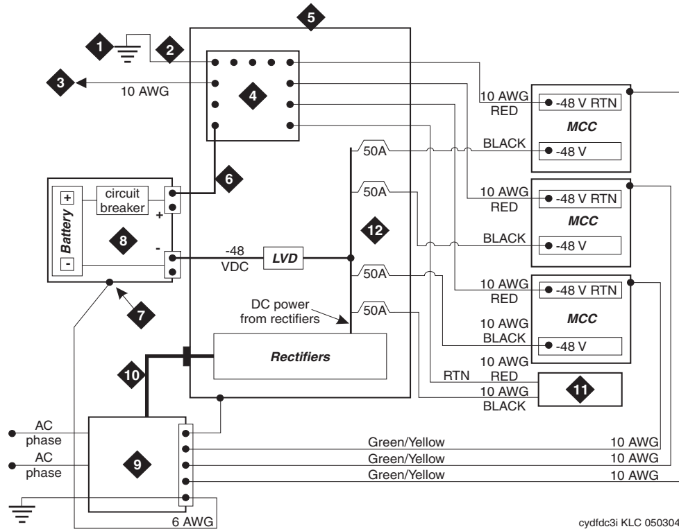
Figure 12: Typical DC power layout for a G650
