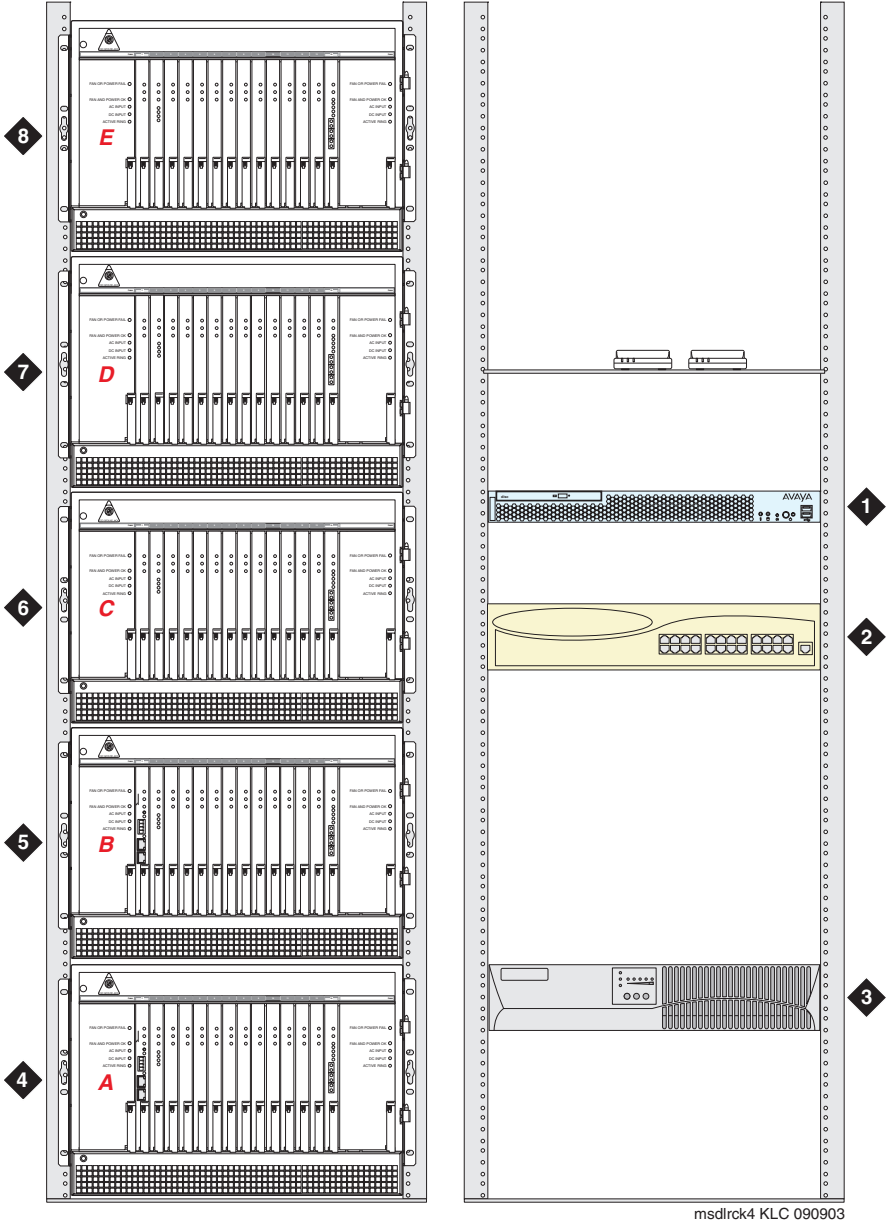
Figure 2: G650 Media Gateway stack (A through E) that is installed next to the server rack
