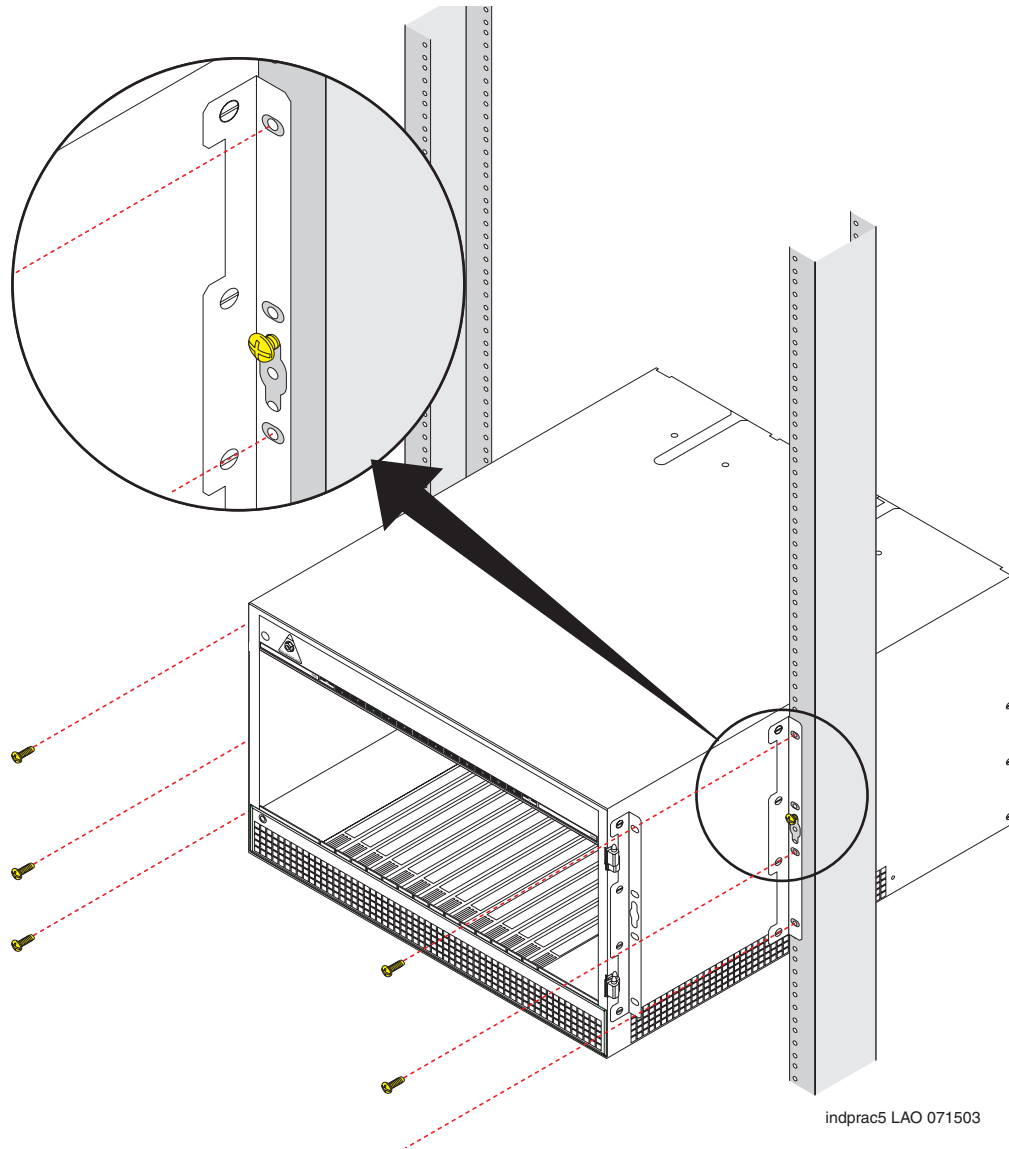
Figure 7: Mounting the media gateway
