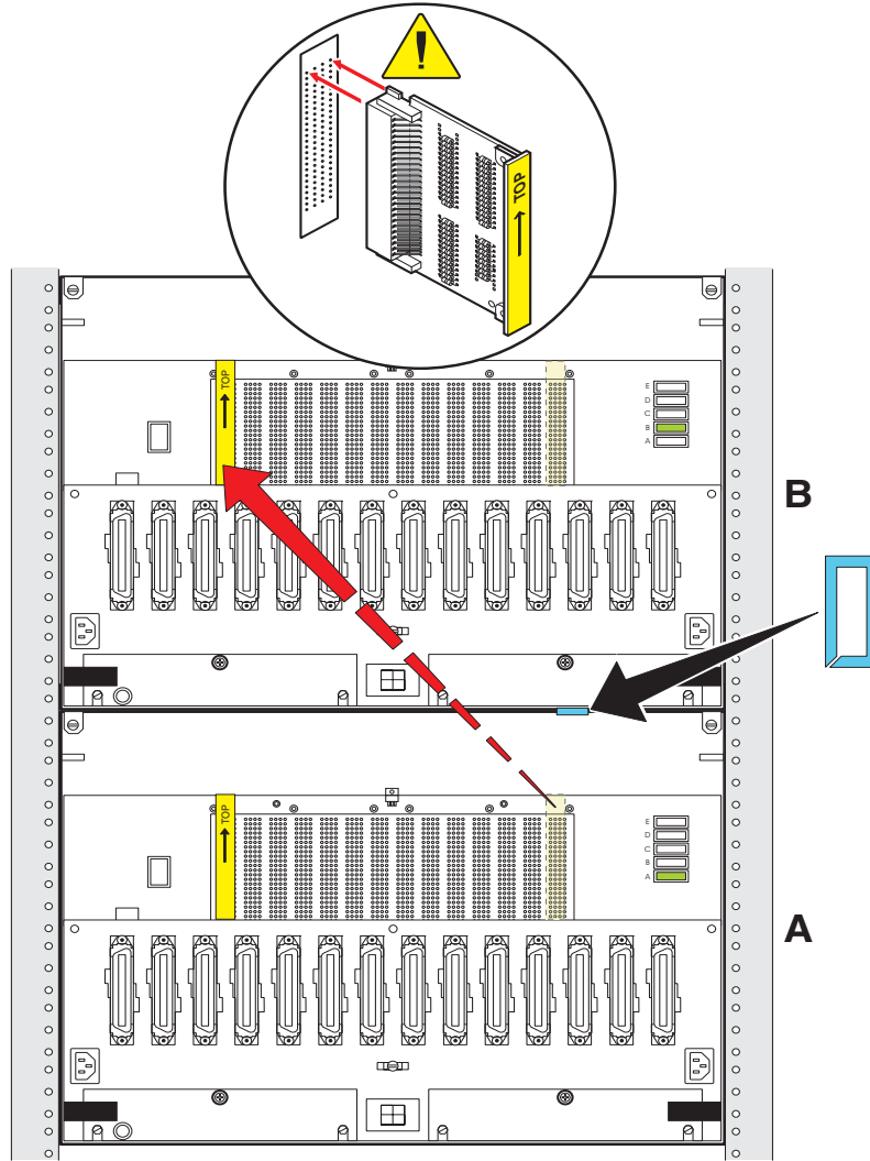
Figure 16: G650 TDM/LAN cable installation (part 3)
