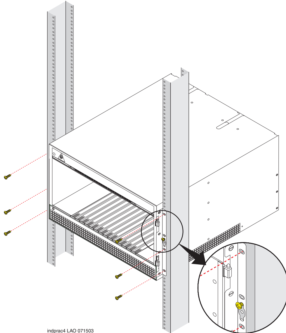
Figure 6: Placement of the holes on the rack and the first mounting screws
