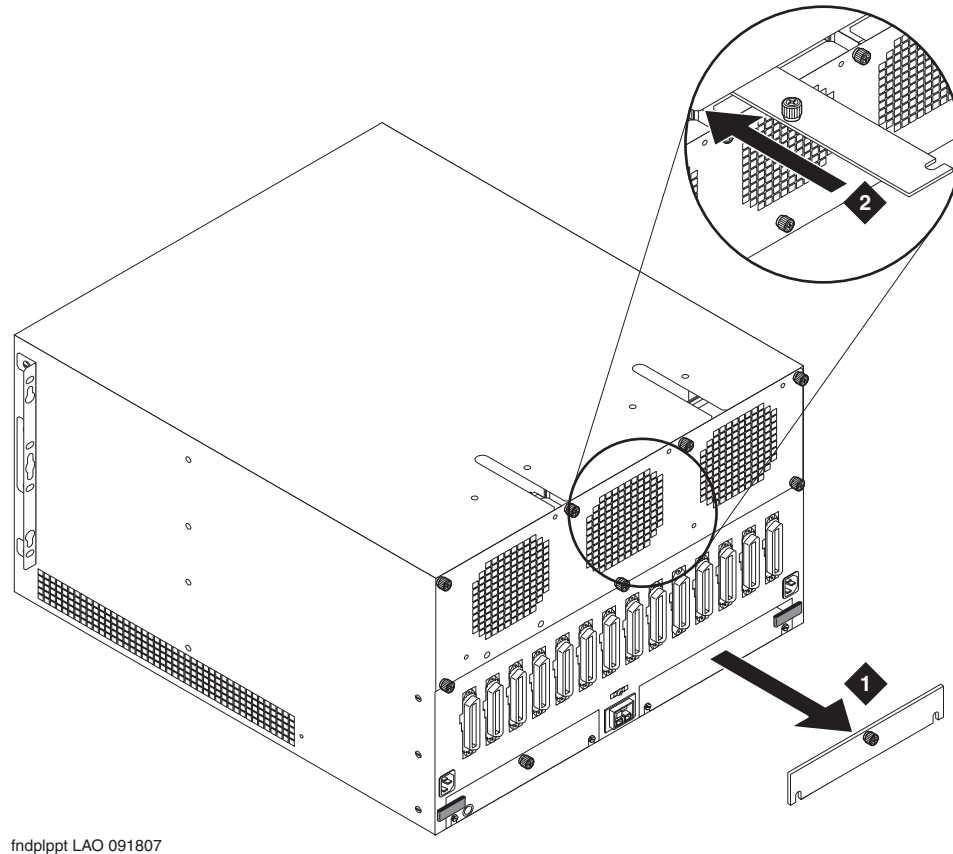
Figure 5: Replacing the fan assembly
