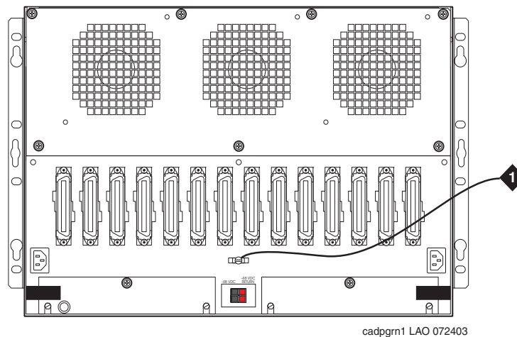
Figure 10: Grounding for a single G650 Media Gateway
