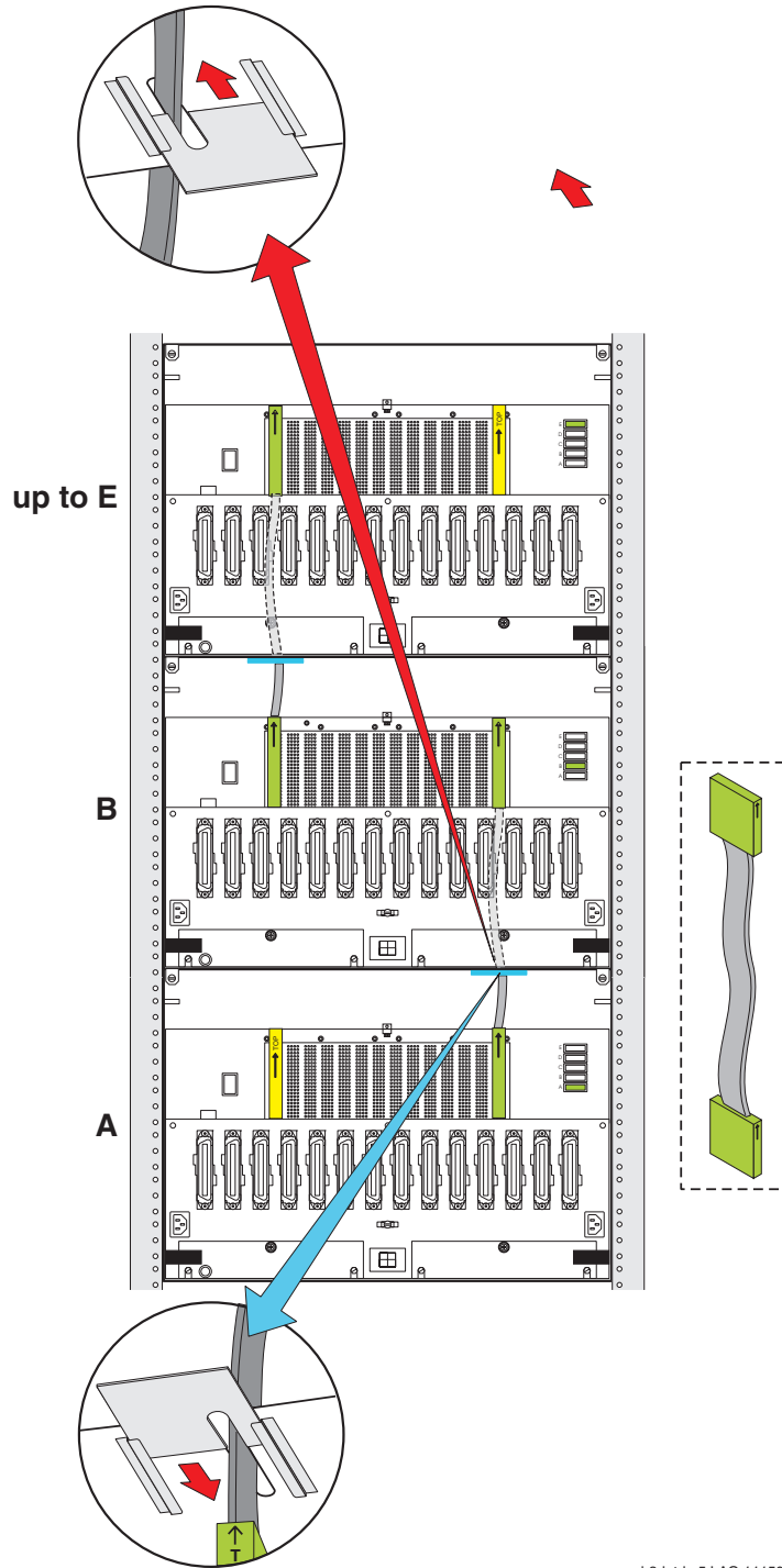
Figure 18: G650 TDM/LAN cable installation (part 5)
