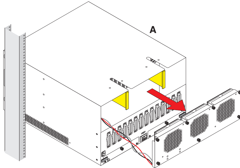
Figure 14: G650 TDM/LAN cable installation (part 1)
