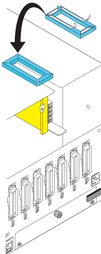
Figure 15: G650 TDM/LAN cable installation (part 2)
