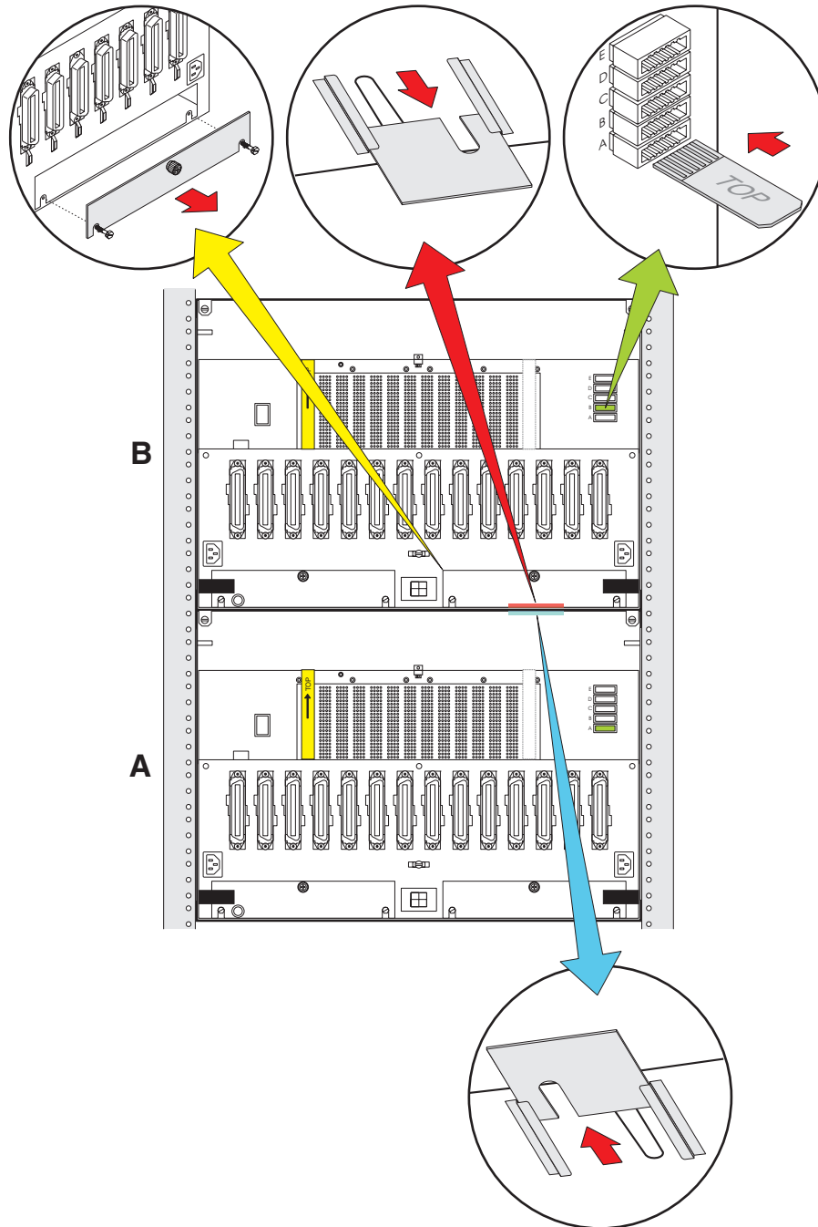
Figure 17: G650 TDM/LAN cable installation (part 4)
