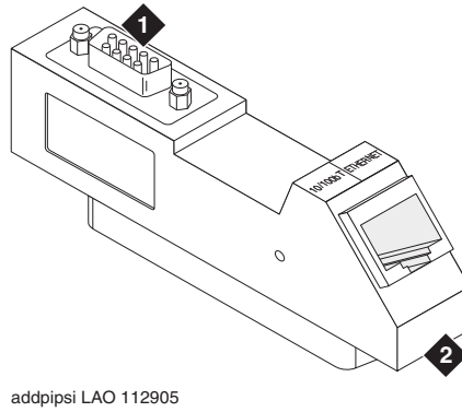
Figure 20: G650 Media Gateway IPSI adapter
