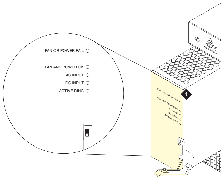
Figure 13: Power supply for the G650 Media Gateway
