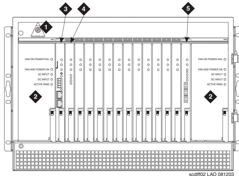
Figure 19: Front view of a G650 Media Gateway
