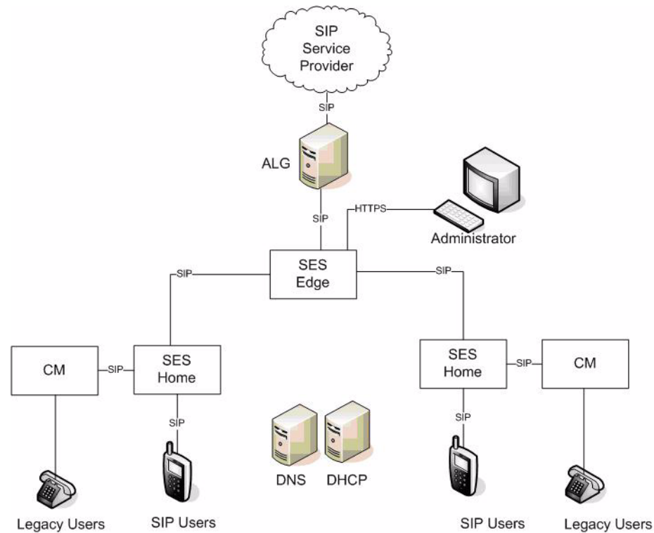
Figure 49: Multi-home multi-Communication Manager configuration
