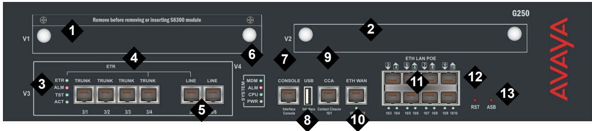
Figure 9: The Avaya G250 analog Media Gateway Chassis,
