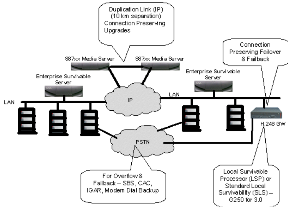
Figure 74: Release 3.0 system example
