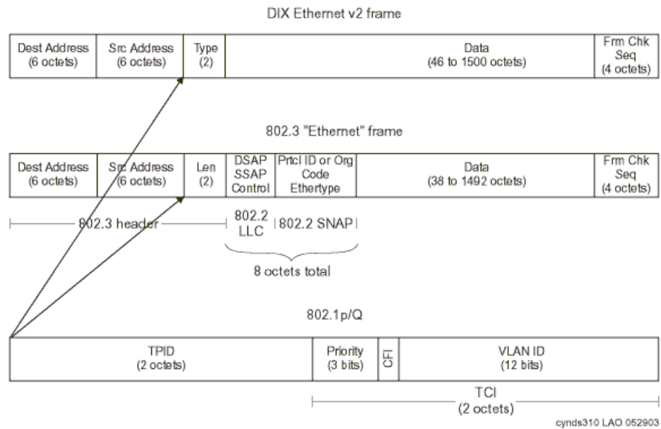
Figure 85: 802.1Q tag
