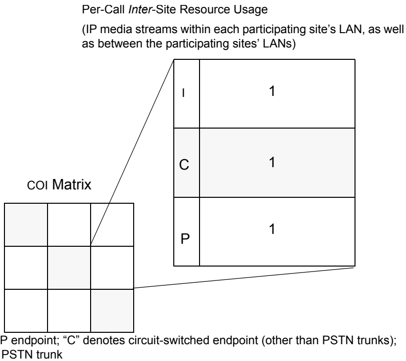
Figure 67: Required number of bidirectional IP media streams for inter-site calls
