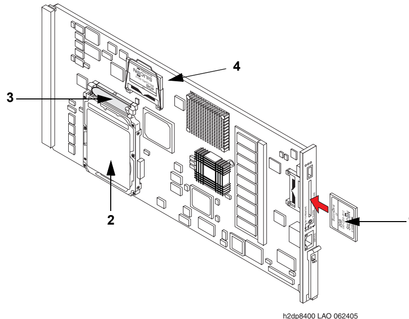
Figure 17: TN8400AP circuit pack (S8400 Server)
