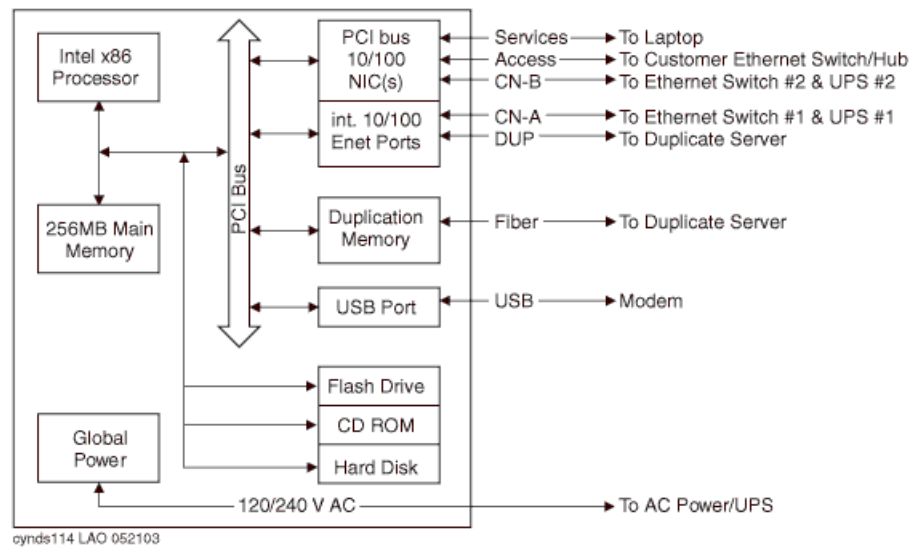
Figure 19: Avaya S8700-series Server schematic
