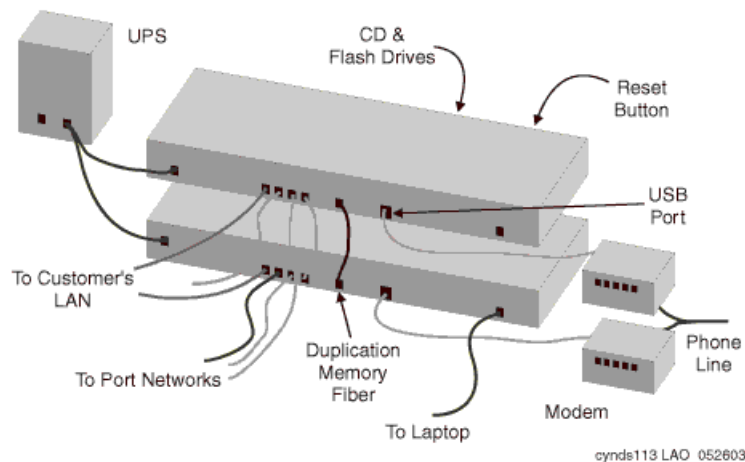
Figure 18: Avaya S8700 external features
