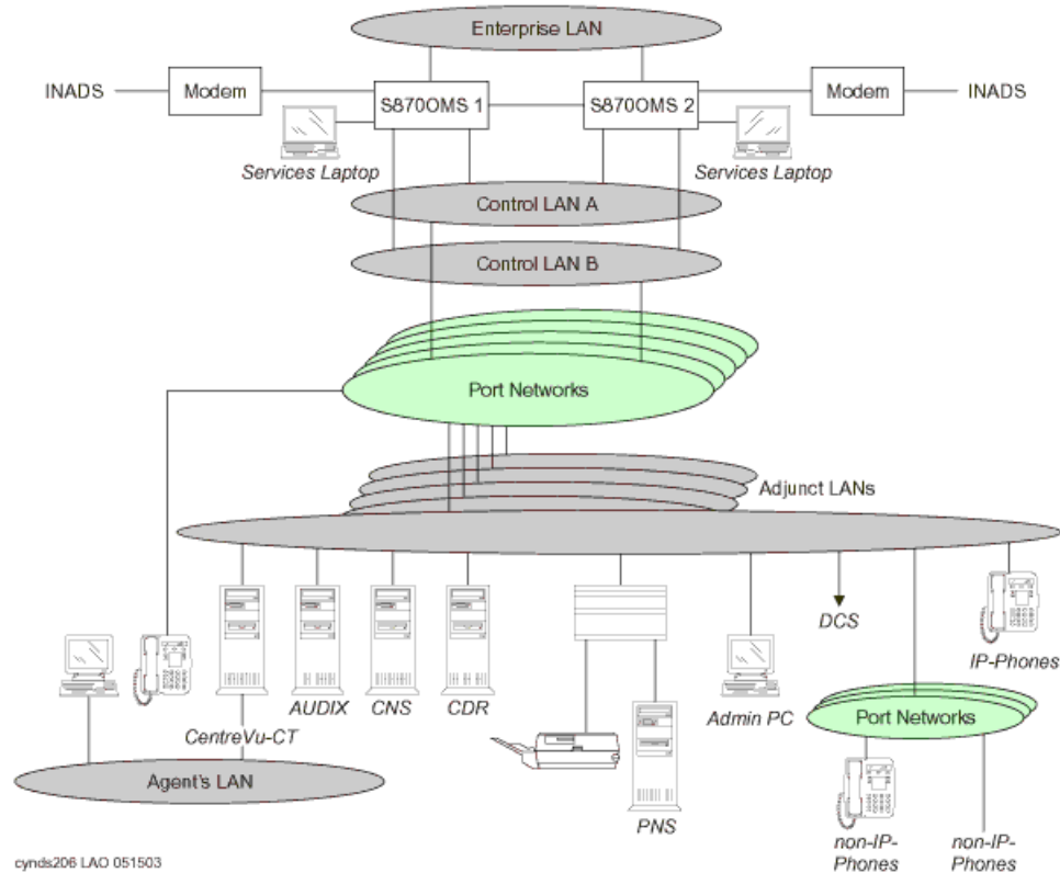
Figure 68: Avaya S8700-series Server with an Avaya MCC1 or an SCC1 Media Gateway
