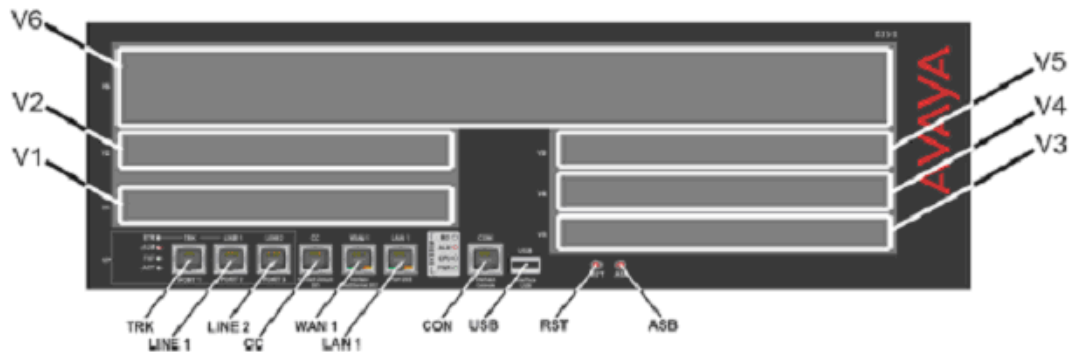
Figure 8: G350 chassis
