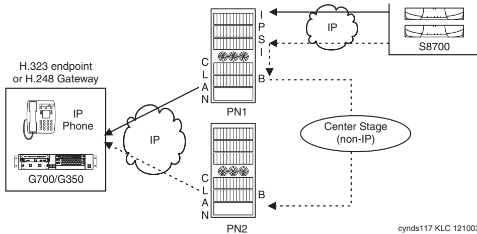
Figure 22: S8700-series / MCC1 signaling path
