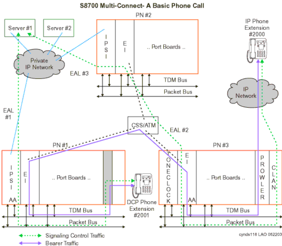
Figure 23: S8700-series fiber-PNC — a basic phone call
