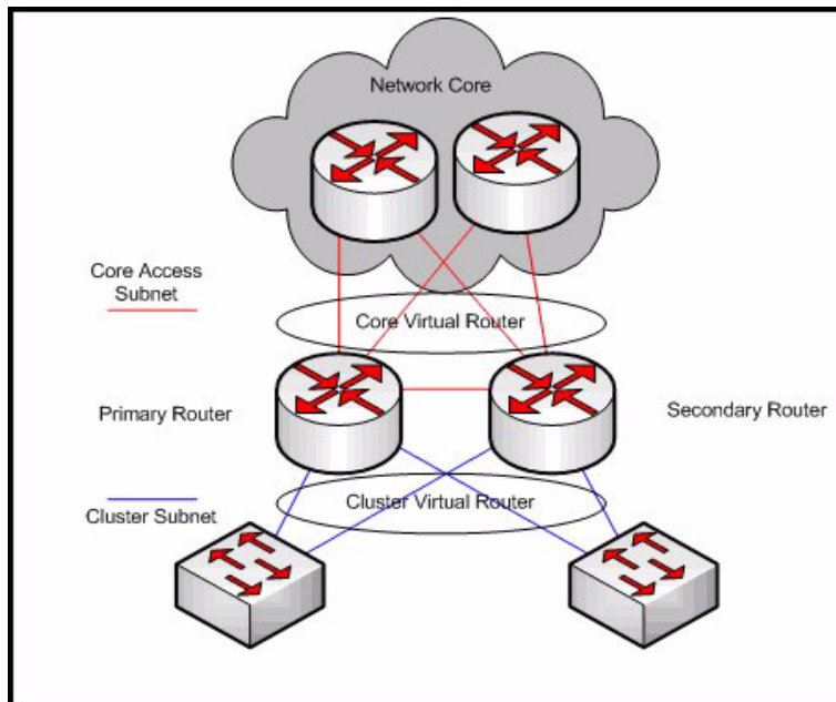
Figure 84: VRRP configured for Core Access
