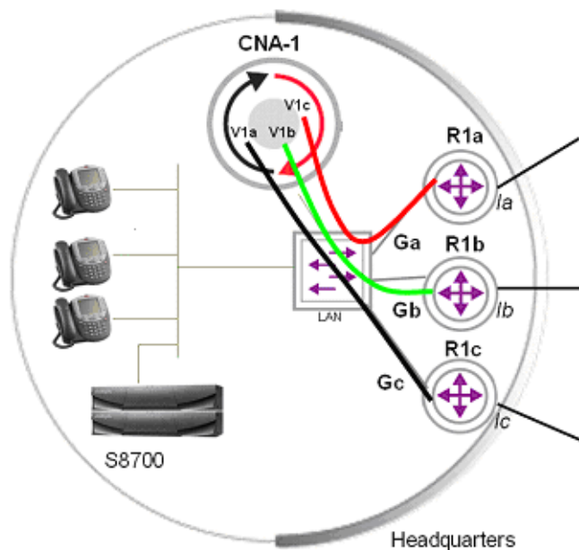
Figure 90: Headquarters CNA deployment – Measurement plane
