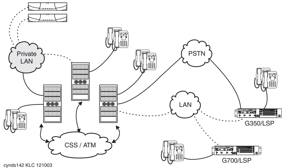
Figure 45: S8700 / G700 / G350 system with Local Survivable Processors
