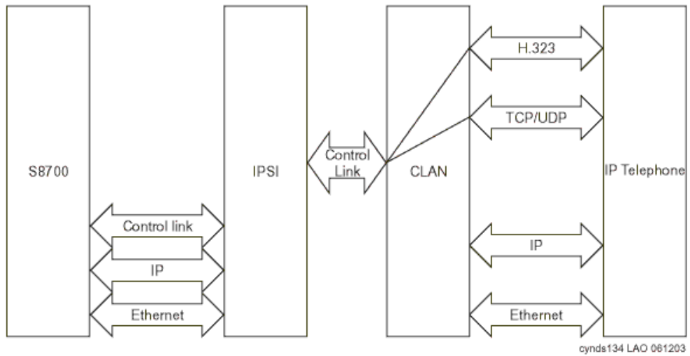
Figure 40: Signaling flow
