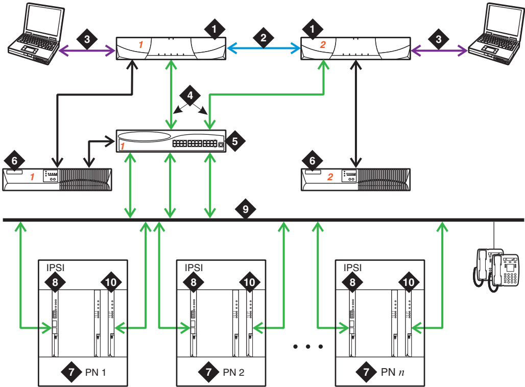
Figure 32: S8700 IP-PNC standard configuration
