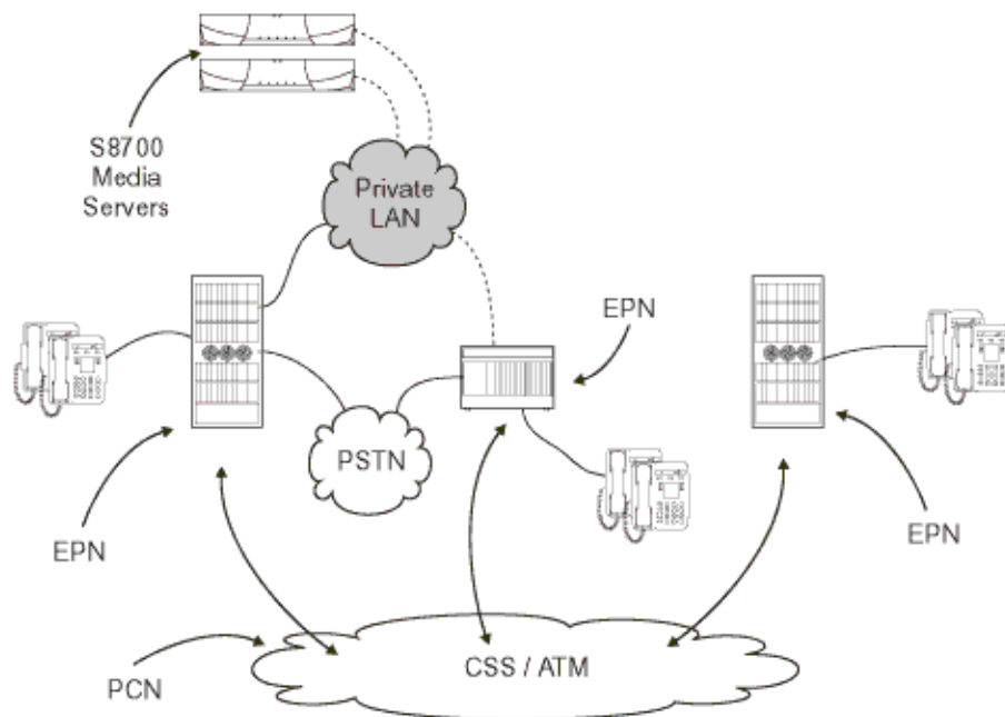
Figure 42: S8700-series Servers (fiber-PNC configuration)
