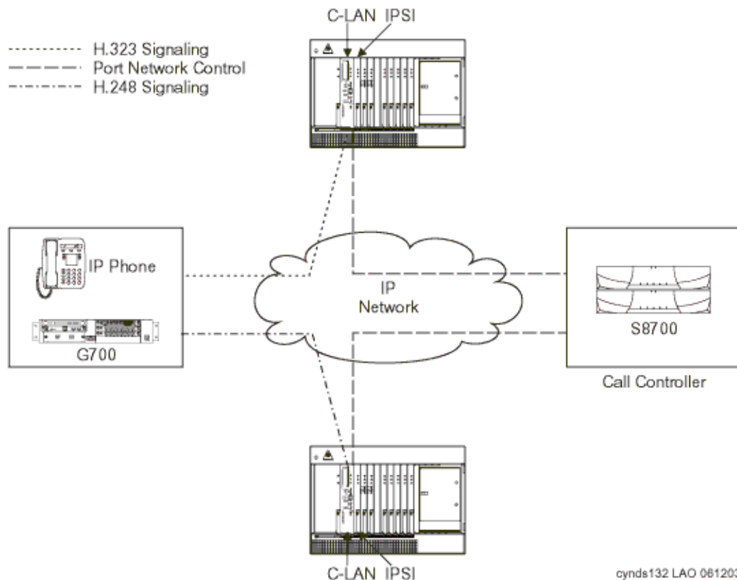
Figure 38: Signaling path (S8700 / G650 configuration)
