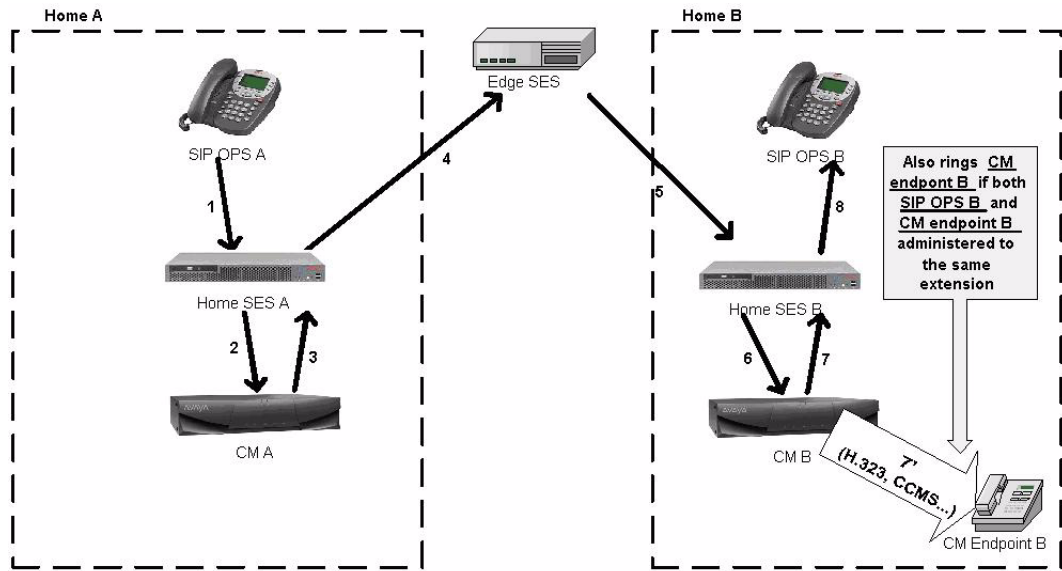
Figure 50: Message flow for multi-home multi-Communication Manager configuration
