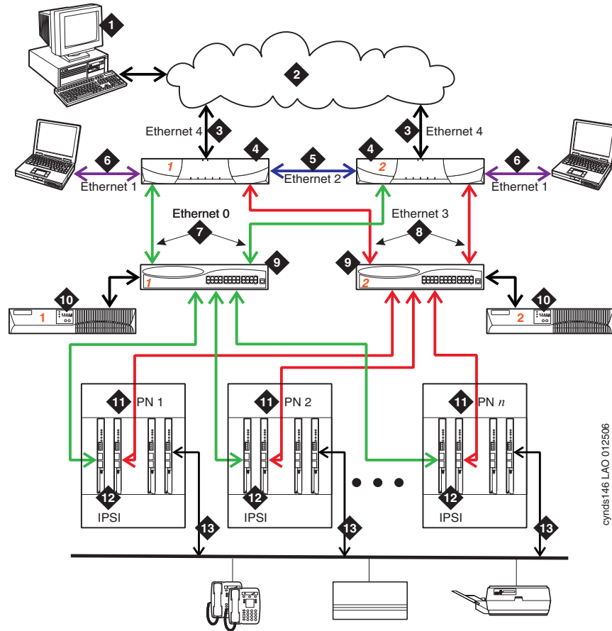
Figure 28: S8700-series fiber-PNC in a high reliability configuration
