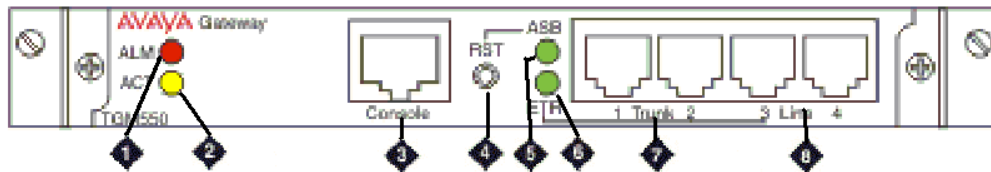
Figure 16: The TGM550 Gateway Module
