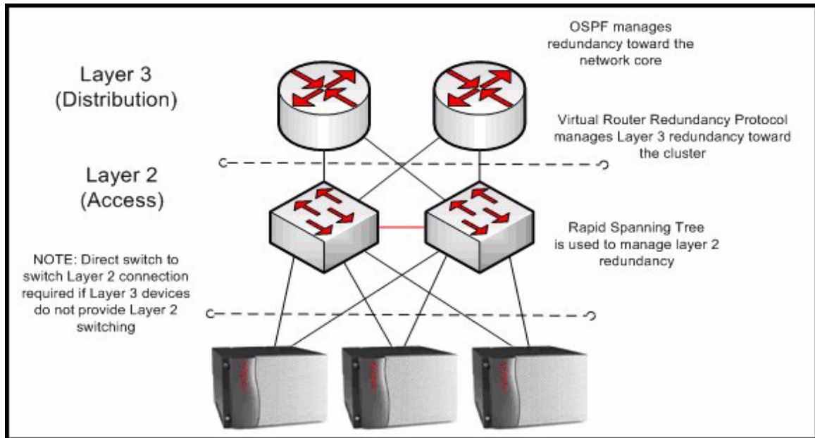
Figure 79: Layered Server Cluster Topology
