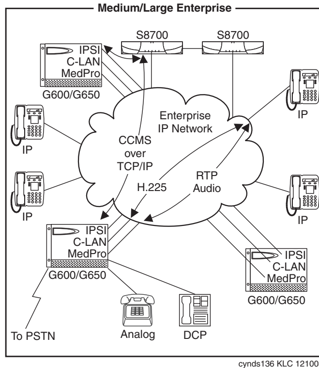
Figure 35: S8700-series IP-PNC system
