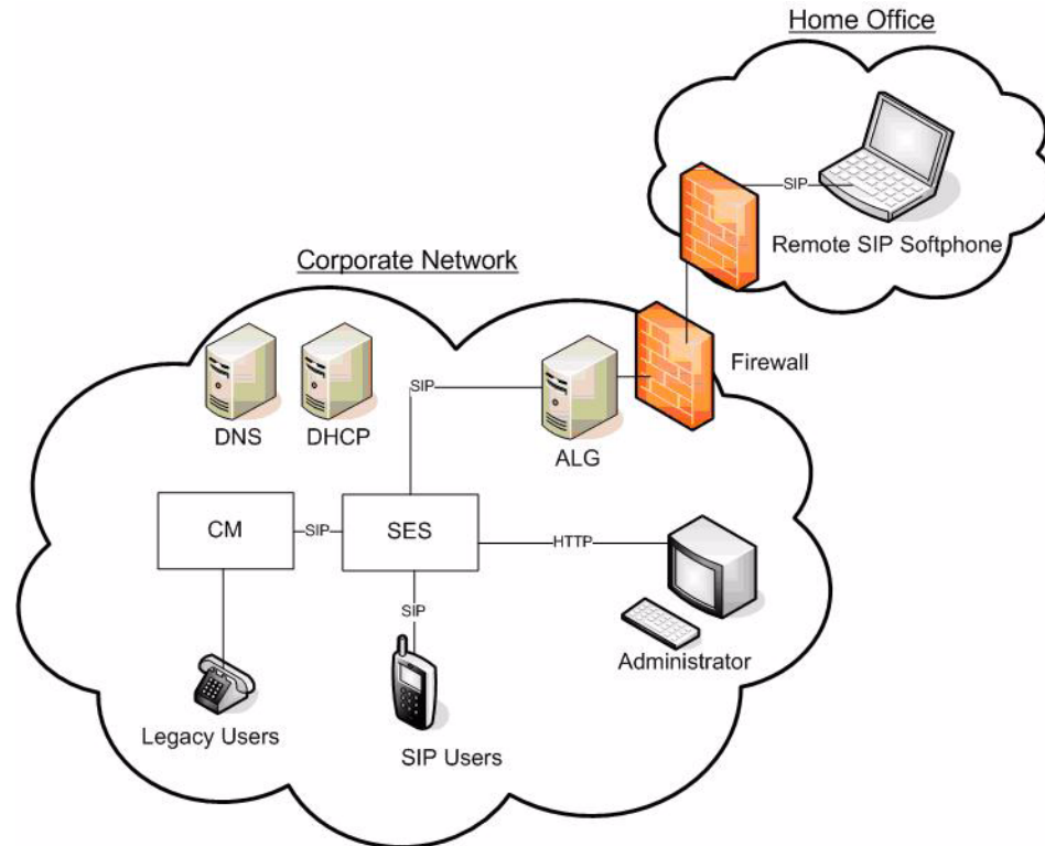
Figure 48: Typical home/edge configuration
