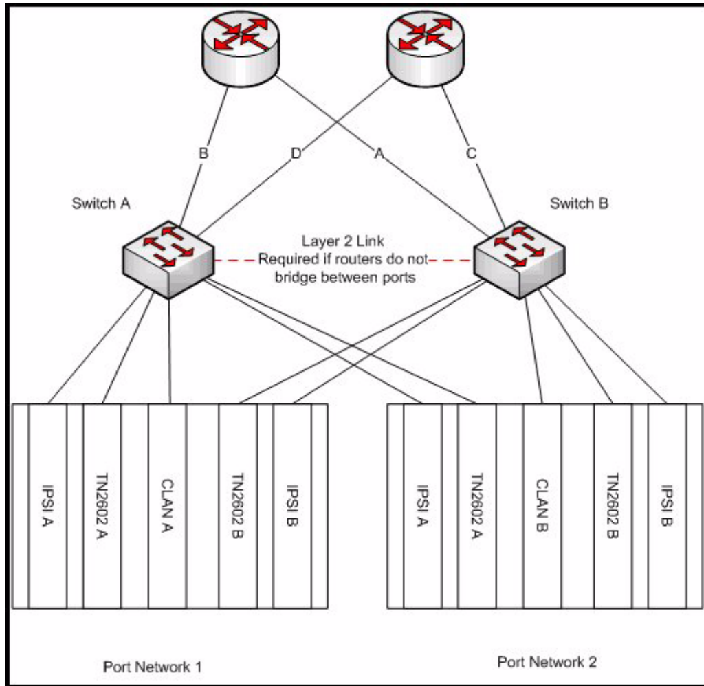
Figure 81: Redundant connections
