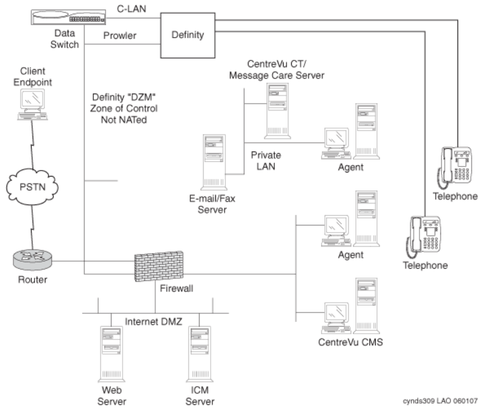
Figure 77: IP Telephony without NAT
