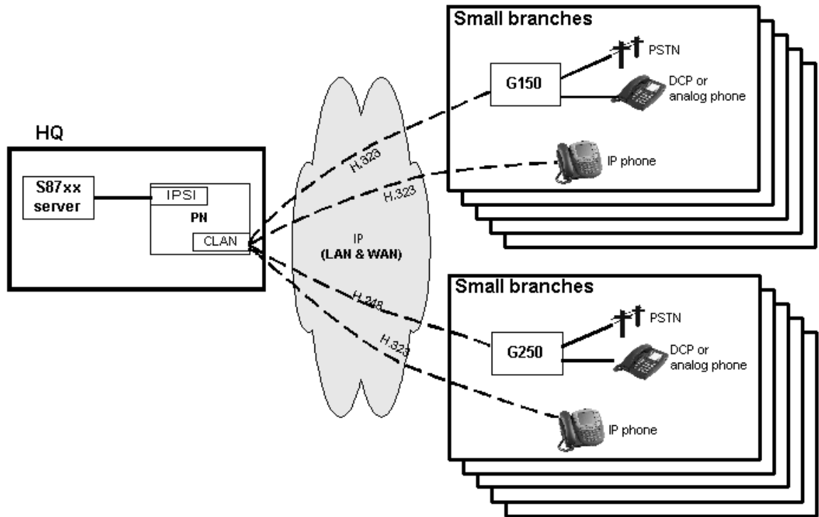
Figure 37: S8700-series with G150/G250 -- large number of remote branches
