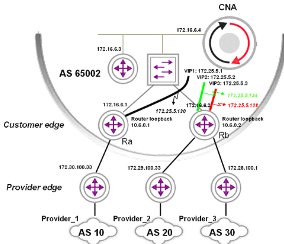
Figure 91: Detailed configuration scenario
