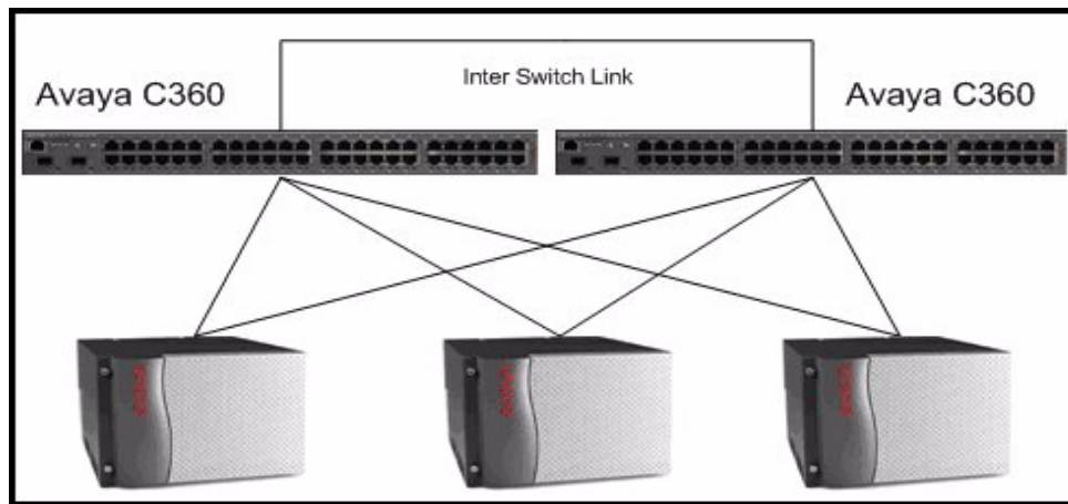
Figure 80: Integrated high density switch topology
