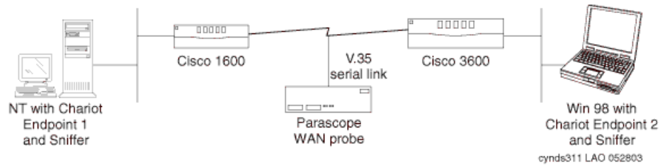
Figure 87: Equipment configuration for RTP header compression test
