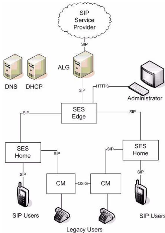
Figure 53: Multi-home multi-Communication Manager configuration with QSIG connection
