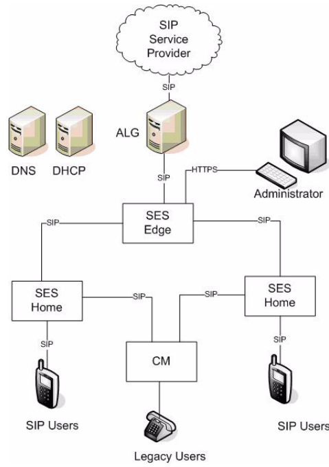
Figure 51: Multi-home single Communication Manager configuration
