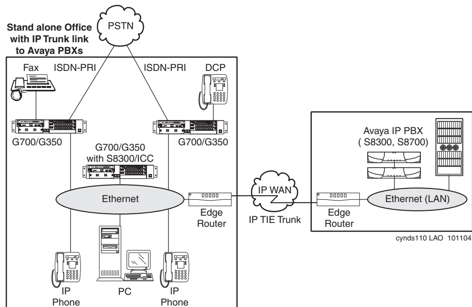
Figure 6: Avaya S8300/G700, G350, or G250 in a stand-alone configuration
