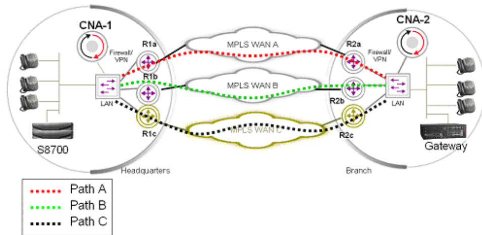
Figure 89: Enterprise example: headquarters and branch connected using 3 diverse paths
