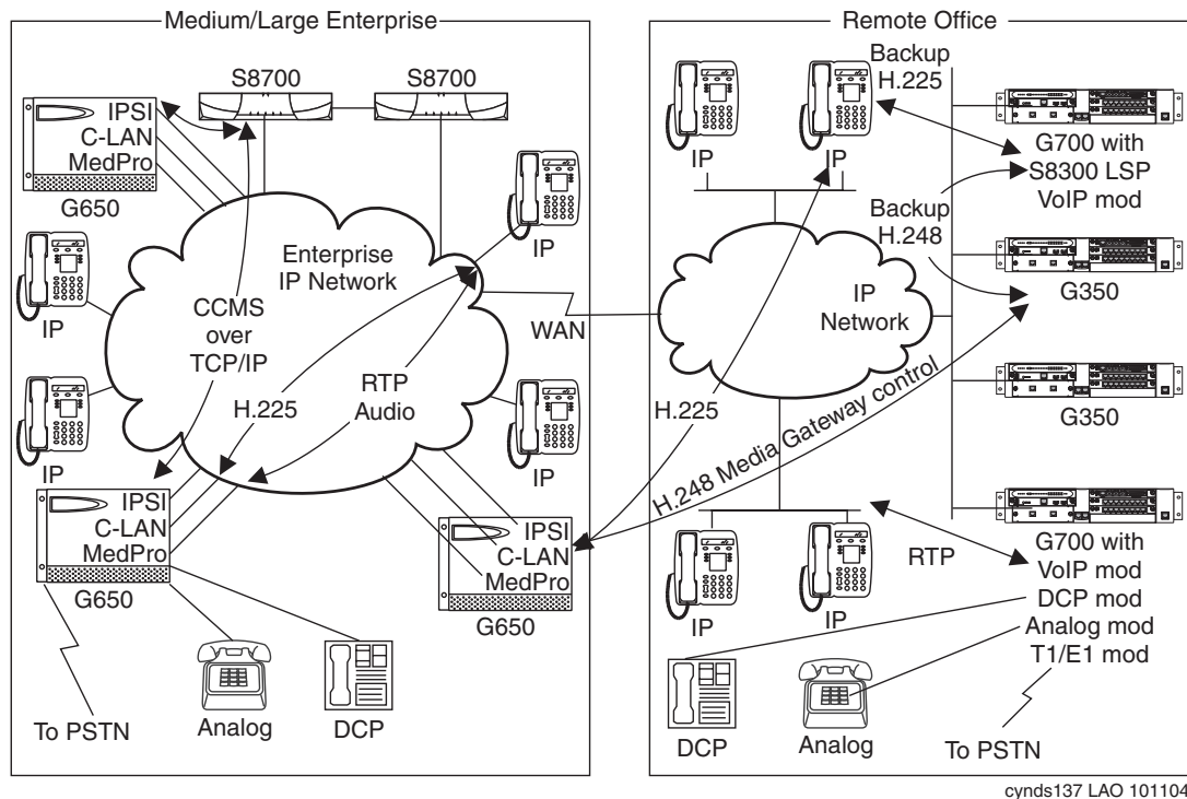
Figure 36: S8700-series IP-PNC with remote G700 or G350s
