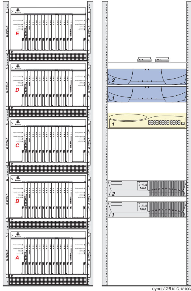
Figure 31: S8700-series Server IP-PNC major components
