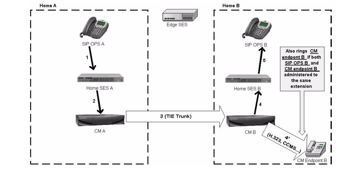
Figure 54: Multi-home multi-Communication Manager configuration with QSIG connection - message flow
