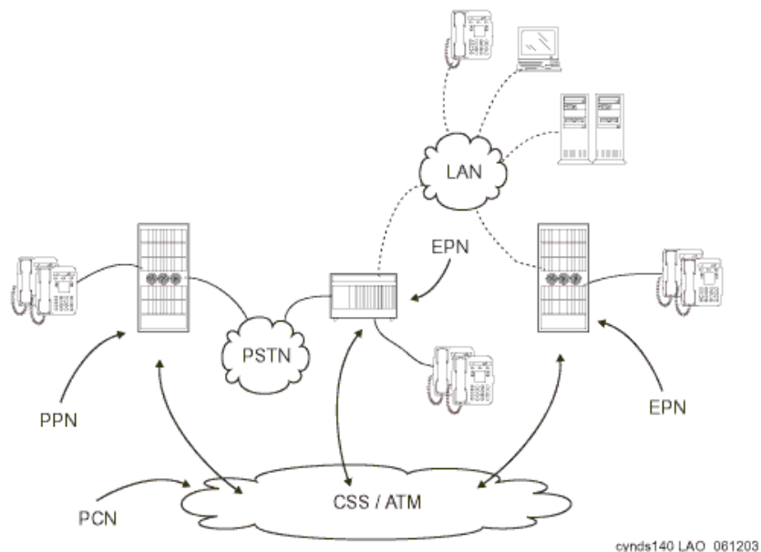
Figure 43: IP-enabled DEFINITY configuration
