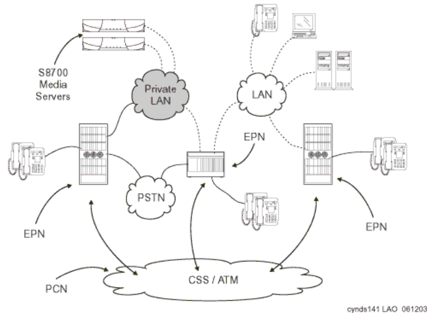
Figure 44: IP-enabling the S8700 fiber-PNC configuration
