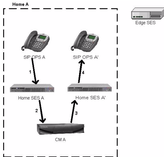
Figure 52: Multi-home single Communication Manager configuration - message flow
