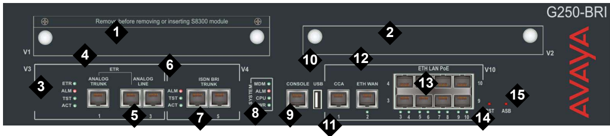
Figure 10: The Avaya G250 BRI Media Gateway Chassis,
