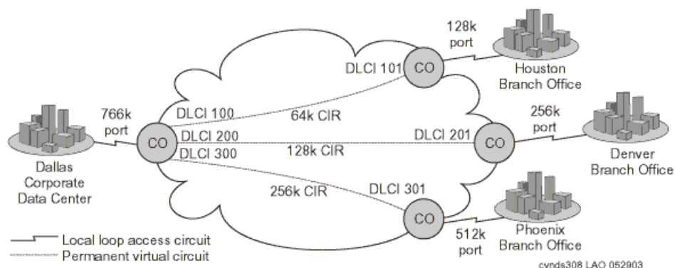
Figure 75: Data-link connection identifiers over an interexchange carrier Frame Relay network
